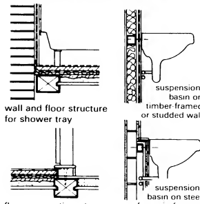
⑭ Important details in damp locations
